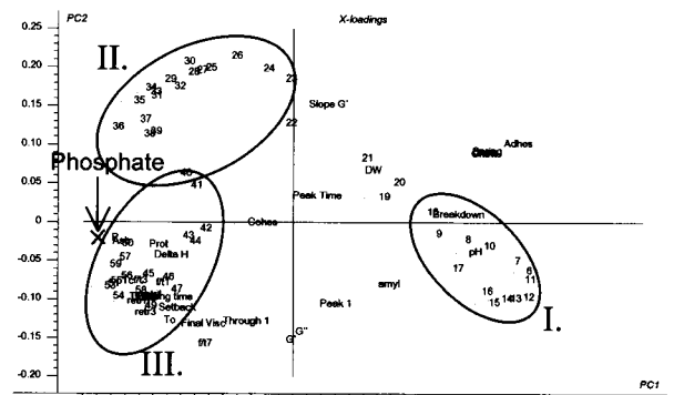
Figure 4. PCA loading plot of all variables.
